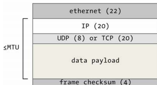
Figure 1. A packet sent using TCP or UDP protocol contains three headers: Ethernet (22 bytes), IP (20 bytes) and TCP or UDP (8 or 20 bytes), a variable-length data payload section and a final frame checksum which is added at the network access layer
